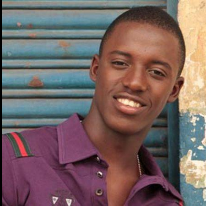
Gappy Ranks
